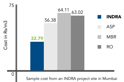
10 Year Life Cycle Cost Comparison - STP (100 KLD)
